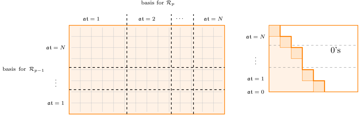
FIGURE 7. Left: The rows and columns of M_p are initially arranged so that the domain and codomain vectors are in increasing and decreasing allow time, respectively. If there are no domain (codomain) vectors having a particular allow time, then the corresponding vertical (horizontal) strip is omitted. Right: After converting to column echelon form, the domain vectors of M_{p,G} need not be in the original ordering. But the codomain vectors are still arranged in decreasing allow time.
