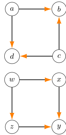
FIGURE 2. Two types of square digraphs.
