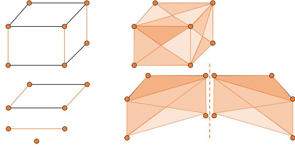
FIGURE 4. Left: \mathfrak{G}_{\square_3}^\delta is (digraph) homotopy equivalent to a point at \delta = 1 , as can be seen by collapsing points along the orange lines. Right: \mathfrak{D}_{\delta, \square_3}^{\text{si}} becomes contractible at \delta = \sqrt{2} , but has nontrivial homology in dimension 2 that persists across the interval [1, \sqrt{2}) .
