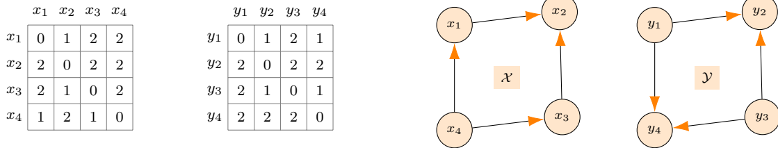
FIGURE 5. Working over \mathbb{Z}/2\mathbb{Z} coefficients, we find that \text{Dgm}_1^{\Xi}(\mathcal{X}) and \text{Dgm}_1^{\mathfrak{D}}(\mathcal{Y}) are trivial, whereas \text{Dgm}_1^{\mathfrak{D}}(\mathcal{X}) = \text{Dgm}_1^{\Xi}(\mathcal{Y}) = \{(1, 2)\} = \{(1, 2)\} .
