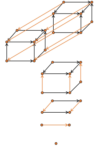
FIGURE 3. Directed d -cubes that are all homotopy equivalent.
